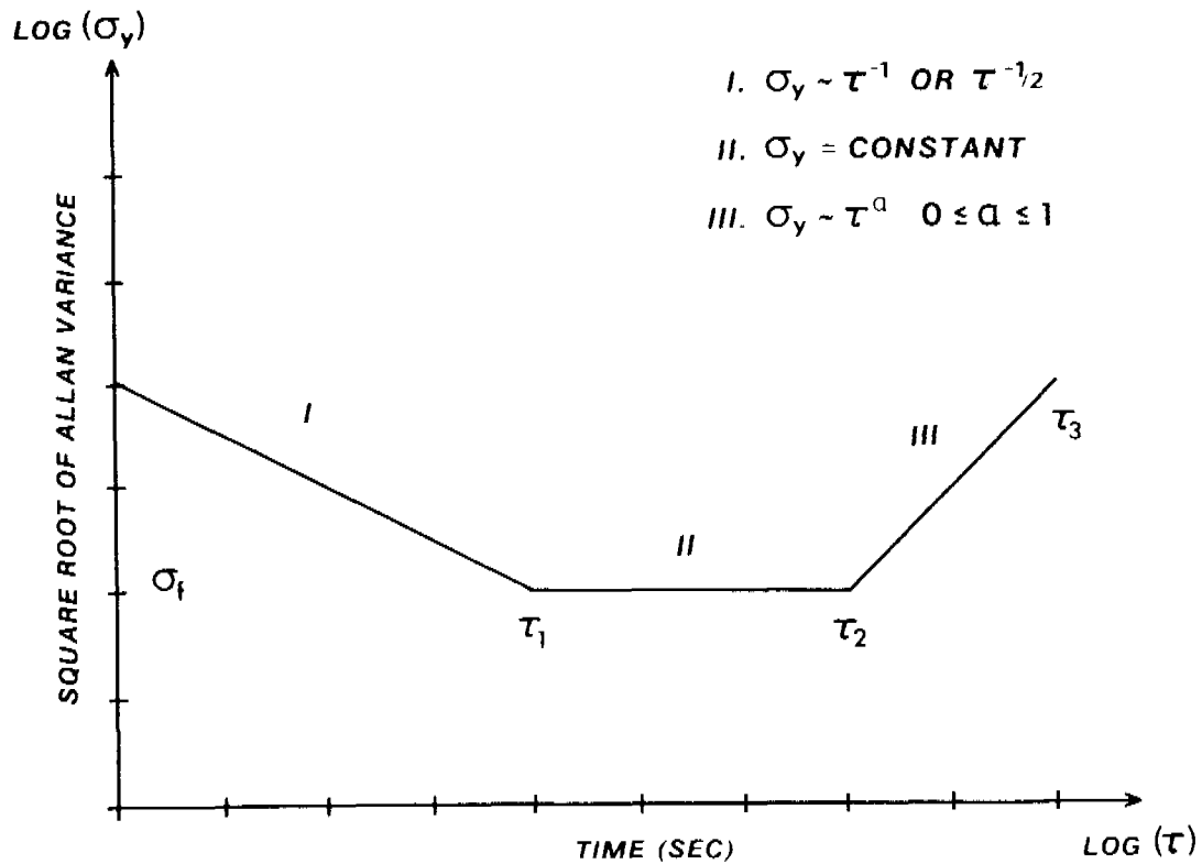
Fig. 1-General frequency stability characteristics
